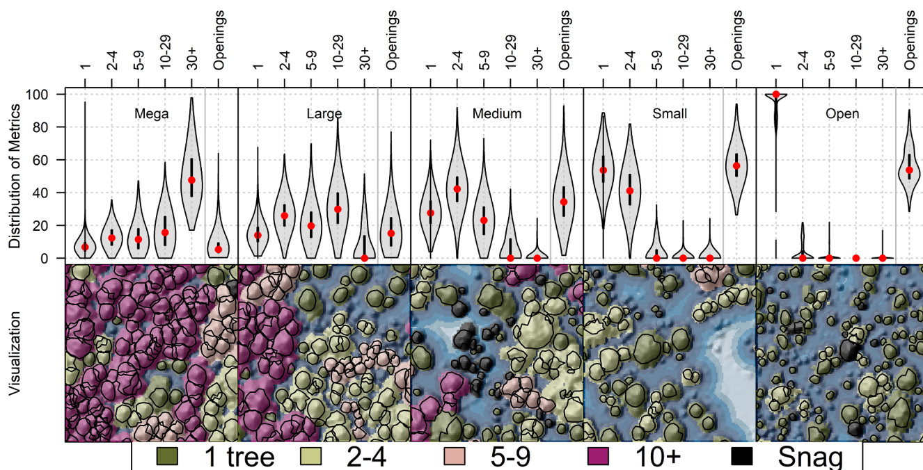
Fig. 2. Visualization of tree approximate object (TAO) clump and opening patterns for 90 m × 90 m areas identified in this study and of the TAO clumping structure classes identified. The distribution of values for the proportion of canopy area in each clump class is shown in violin plots. Names for each class reflect the dominant tree clump sizes: open area dominated by individual TAOs, small clumps (2 to 4 TAOs), medium clumps (2 to 4 and 5 to 9 TAOs), large clumps (10 to 29 TAOs), and mega clumps (≥ 30 TAOs). Classes were defined by the percentage of canopy cover > 2 m in each clump size and percentage of open space in each 90 × 90 m grid cell. Clump size ranges for each violin plot shown above figure. Black lines show the modeled TAO canopy boundaries. Violin plots show the distribution of values for grid cells in each tree clump size class, with dots depicting the mean value, lines showing the extent of the 25th to 75th percentile range, and width showing the frequency of values.
