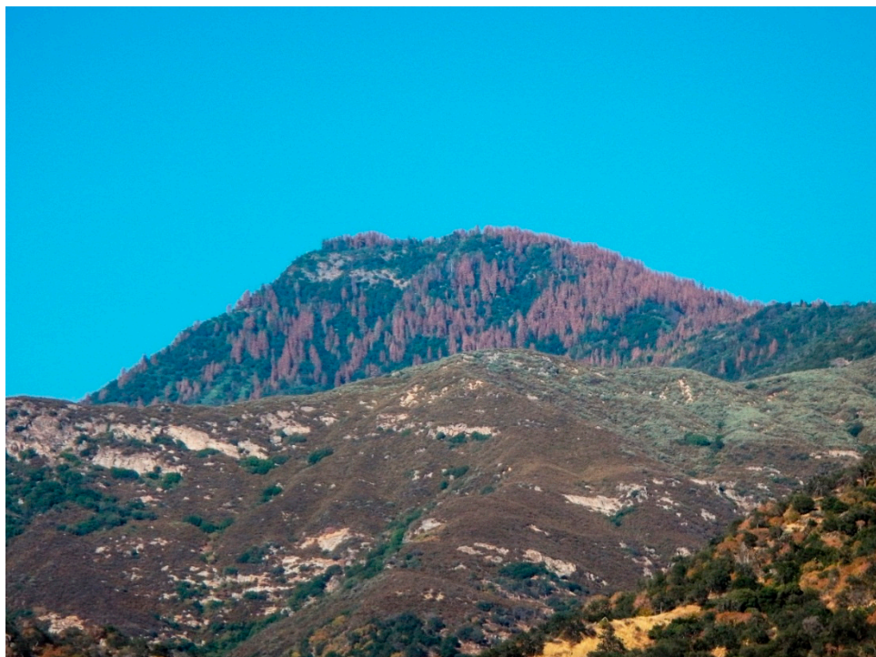
Figure 4. Severe die-off of Pinus ponderosa in a mixed conifer forest on the north-facing slope of Case Mountain in the southern Sierra Nevada Range, California, in July 2016 (lower slope dominated by chaparral that experienced little or no die-off). This followed a near-record-breaking drought during 2012–2014, which is thought to have been exacerbated by anthropogenic warming both directly due to physiological stress and indirectly through enhanced pathogen activity. Parsing out the role of global warming is complicated by the fact that these forests have substantially higher tree density due to 125 years of fire suppression, a perturbation to the natural regime of fires every 10–20 years (photo by Jon E. Keeley).
